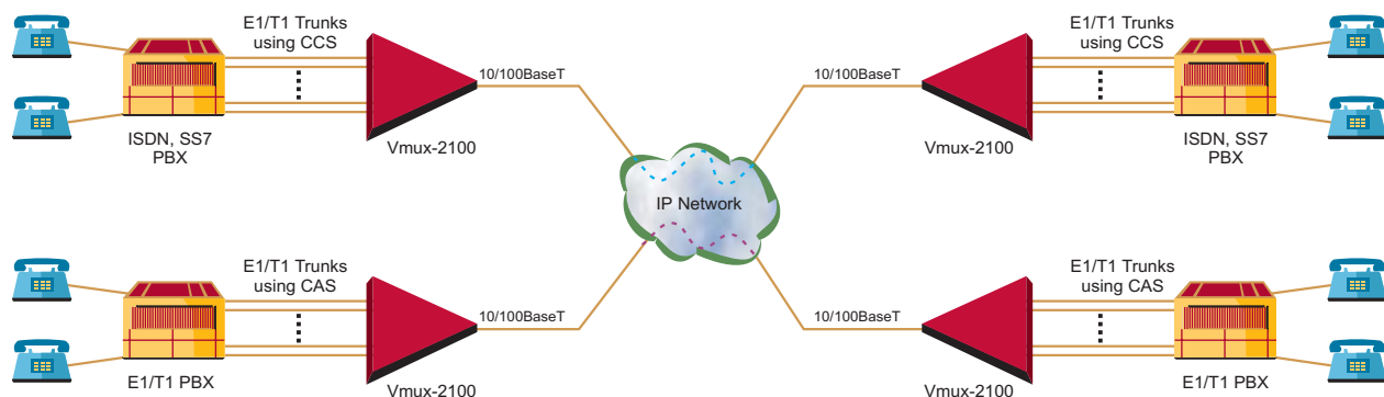
Figure 2. Vmux-2100 Transmitting Compressed Voice over IP, Including Transparent Transmission of CCS and CAS Signaling
