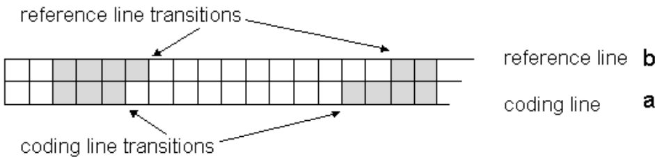
Figure 10: Two dimensional compression.
